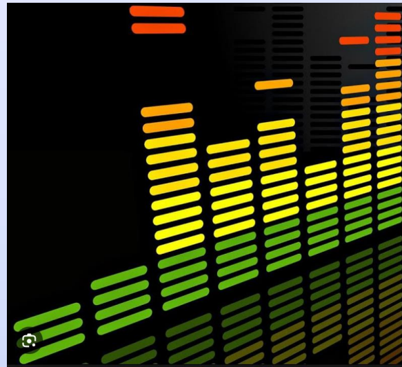
Meta MusicGen
